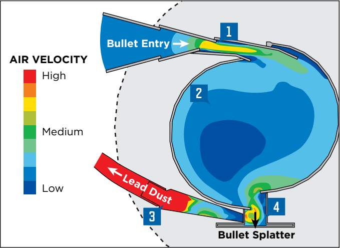
Side view of Vortex air flow analysis.
